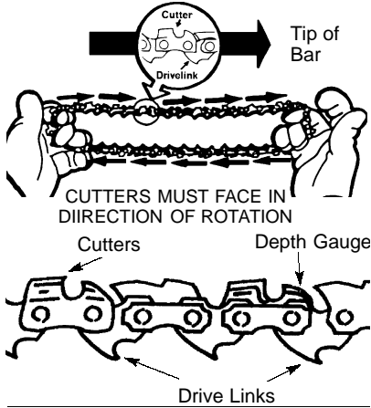
Mount the Bar
